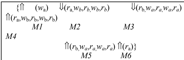
Fig 1. March BDN O(n) = 22n
