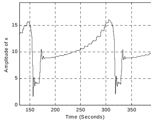
Fig.8 Variable's x oscillations get for T_1=50s, T_2=100s, \tau_1=20s, \tau_2=10s, \tau_3=15s
