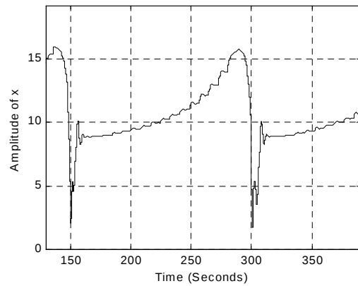
Fig.7 Variable's x oscillations get for T_1=50s, T_2=100s, \tau_1=20s, \tau_2=0, \tau_3=0
