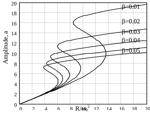
Fig. 4 Resonant curves for different values of the parameter \beta
