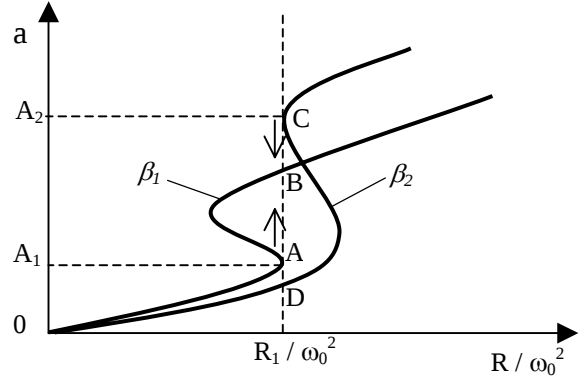
Fig. 3 Explanatory for the resonance jump phenomenon
