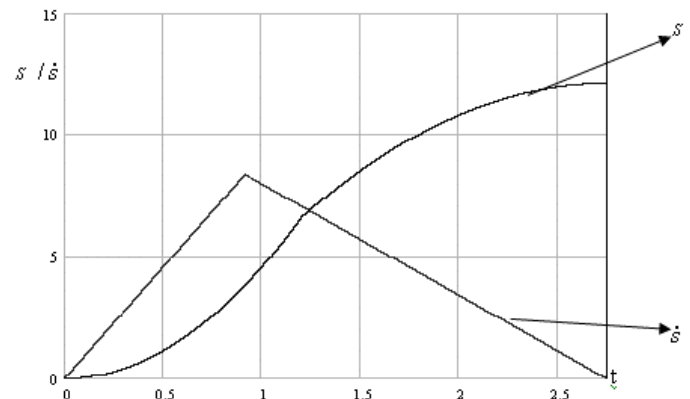
Fig 3.b Simulation results for time-optimal control , type bang-bang ,of robotic arms
