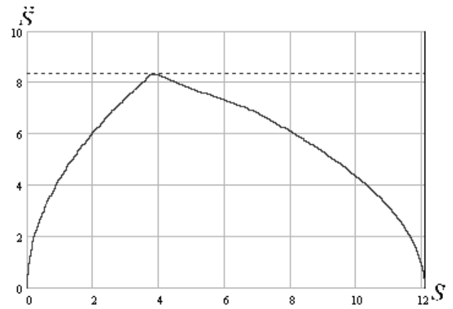
Fig 2.b Simulation results for time-optimal control of robotic arm with two rotational joints
