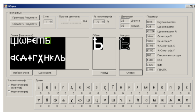
Figure 4. Feature extraction module
