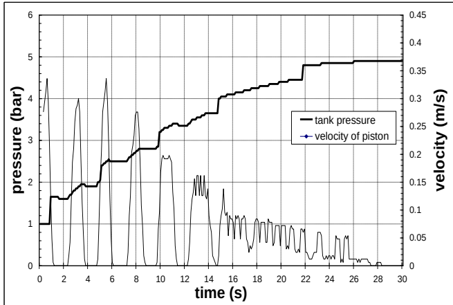
Fig. 12. Velocity of piston and tank pressure
