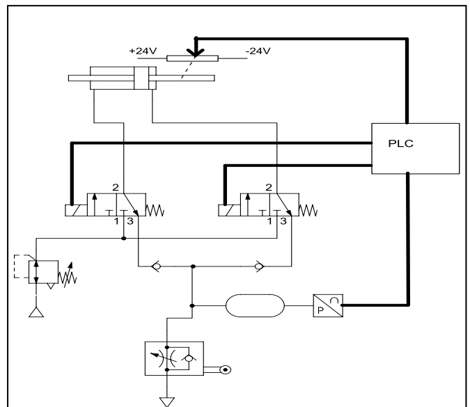
Fig. 8. Pneumatic, measurement and control scheme of experimental installation
