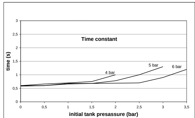
Fig. 14. Time constant value versus initial reservoir pressure
