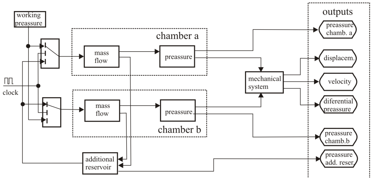
Fig. 1. Simplified block diagram of the simulation
