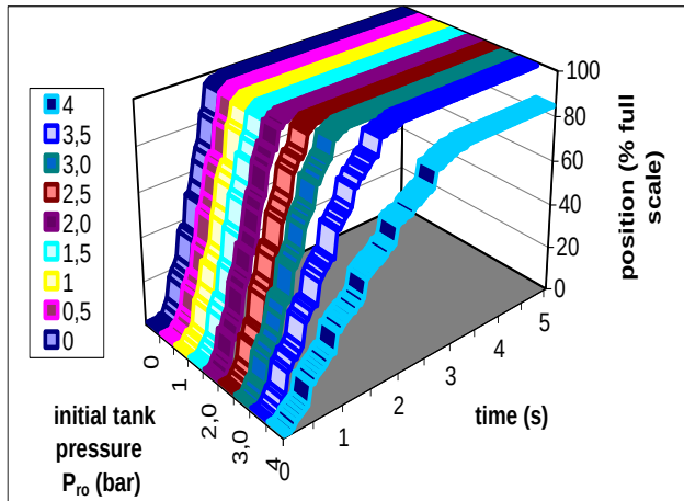
Fig. 13. Position of piston versus initial reservoir pressure
