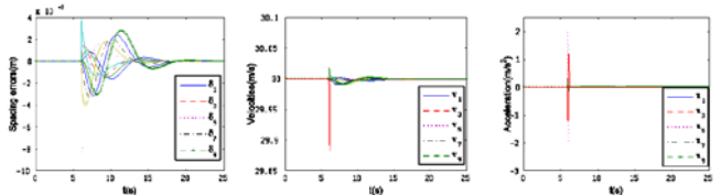
Fig. 6. Sensitivity of the proposed controller to the influence of disturbances.
