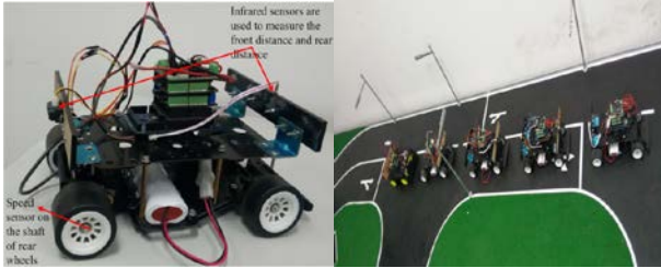
Fig. 7. (a) Arduino car; (b) Arduino platoon system.
