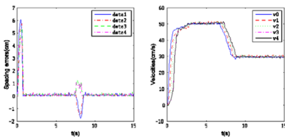
Fig. 8. (a) Spacing errors; (b) Velocities.
