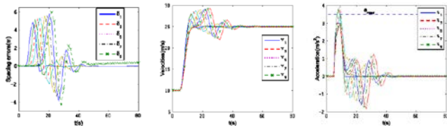
Fig. 3. (a) Spacing errors; (b) Velocities; (c) Acceleration.
