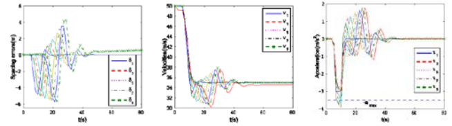
Fig. 5. (a) Spacing errors; (b) Velocities; (c) Acceleration.
