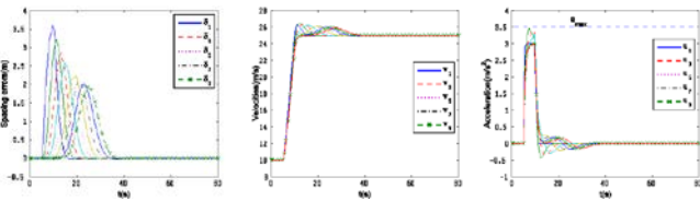
Fig. 2. (a) Spacing errors; (b) Velocities; (c) Acceleration.
