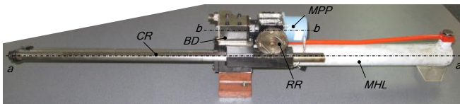
Fig. 9. A view of the system built according to the principle scheme presented in Fig. 7 (variant II)
