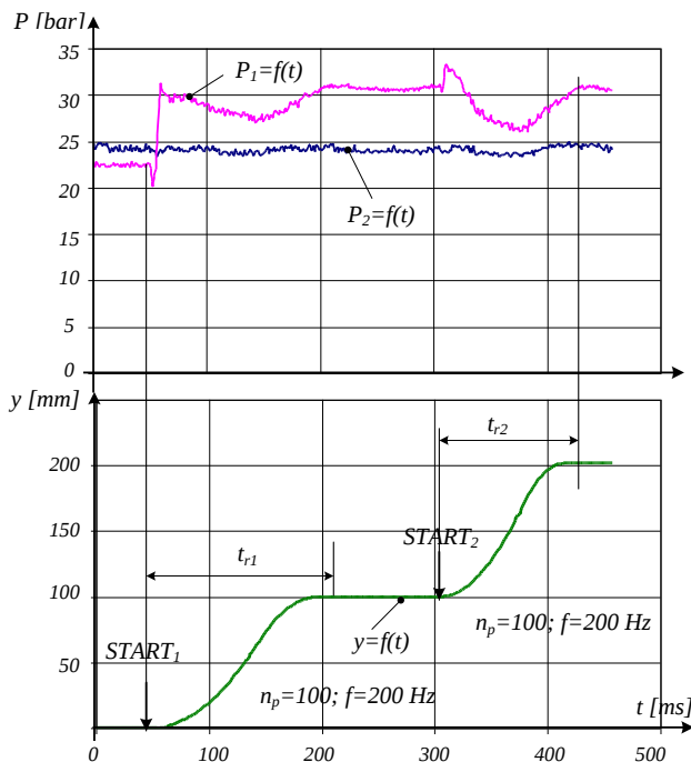
Fig. 16. The experimental results for y_1=100\text{mm} and y_2=200\text{mm}
