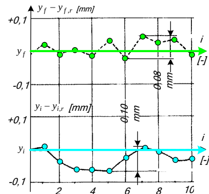
Fig. 14. The results for 20 working cycles
