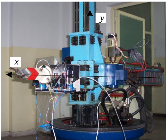
Fig. 18. A view of the hydraulic robot
