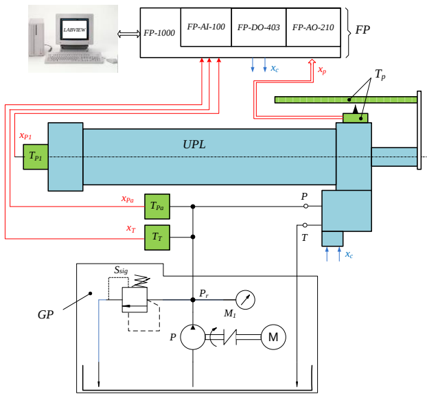
Fig. 12. The functional scheme of the stand for the first variant
