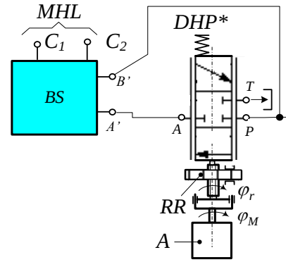
Fig. 7. The principle scheme of the system with one consumer
