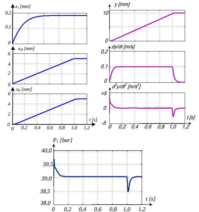
Fig. 11. The results of the simulation
