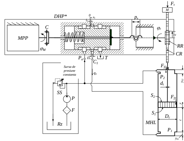
Fig. 10. The principle scheme for the mathematical model
