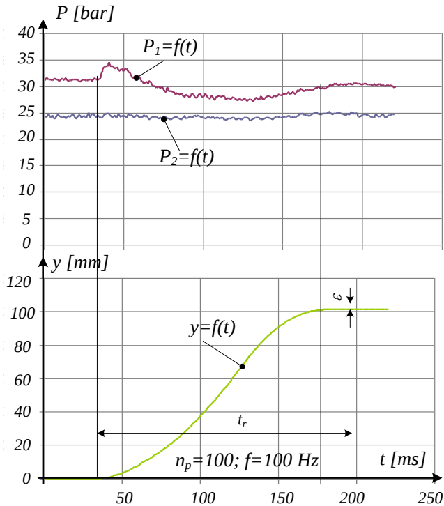
Fig. 15. The experimental results for y=100\text{mm}
