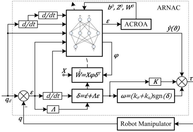
Fig. 3. Structure of ARNAC system.
