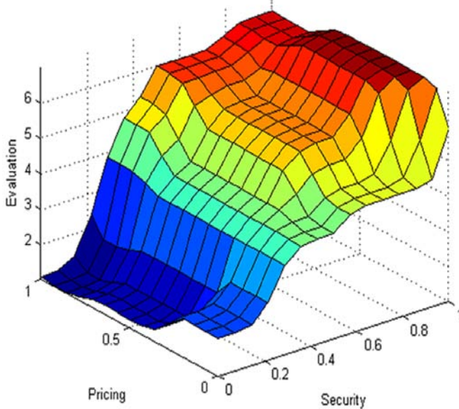
Fig. 4(d). Surface plot for the user's parameters, namely, pricing and security.
