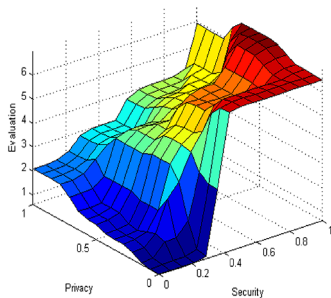
Fig. 4(c). Surface plot for the user's parameters, privacy and security.
