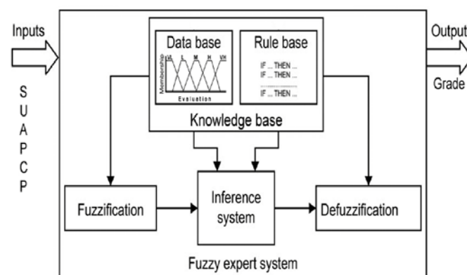
Fig. 1. The generic structure of fuzzy expert system for evaluation of mobile solutions.
