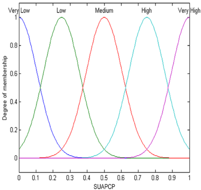
Fig. 2. Membership functions for SUAPCP factors.
