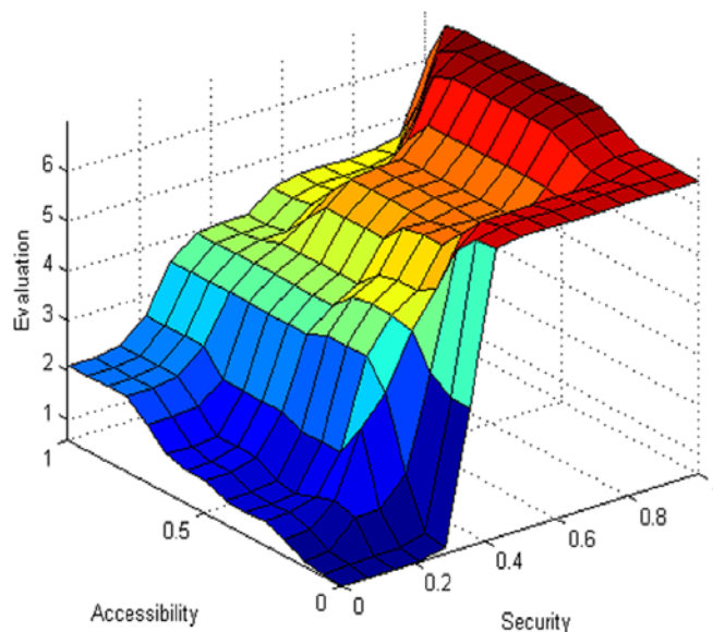
Fig. 4(b). Surface plot for the user's parameters, namely, accessibility and security.
