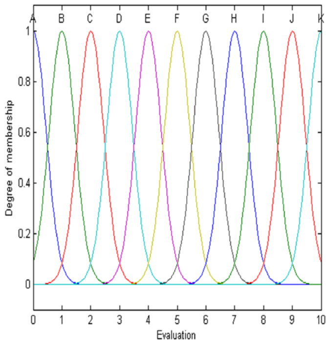
Fig. 3. Membership functions for evaluation of mobile solutions.
