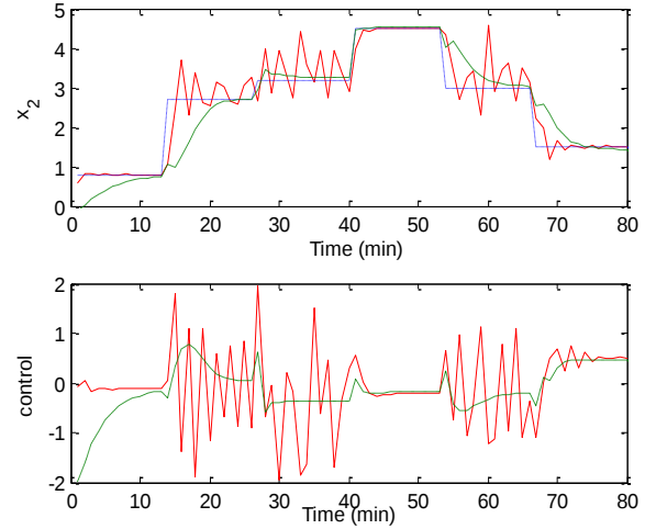
Fig. 7. Closed-loop responses and control inputs moves of CSTR using one controller ((dotted) setpoint; (solid) with K_1 ; (dashed) with K_2 ).
