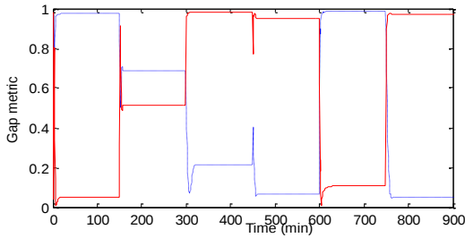
Fig. 3. Calculated gap metrics ((dotted) \delta_1 ; (solid) \delta_2 )
