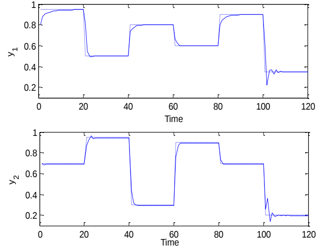
Fig. 8. Closed-loop response of TITO system using three controllers.
