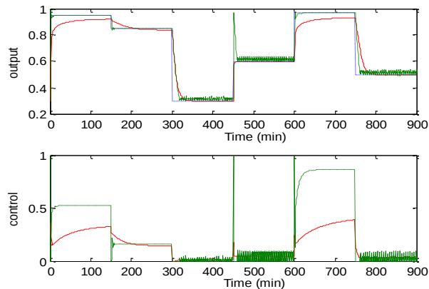
Fig. 4. Closed-loop responses and control inputs moves of CSTR using one model ((dotted) setpoint; (solid) with K_1 ; (dashed) with K_2 ).
