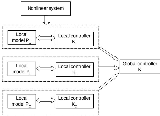
Fig. 1. Schematic diagram of the multimodel control.
