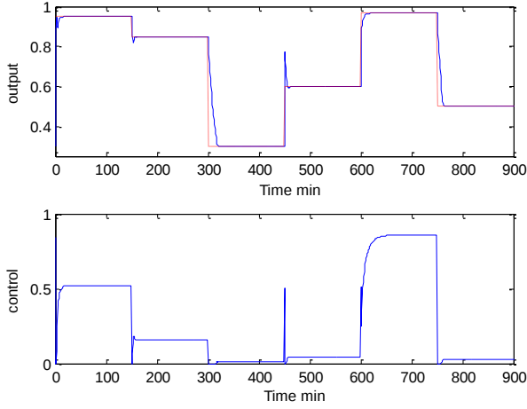
Fig. 2. Closed-loop response and control input moves of the CSTR using two controllers.
