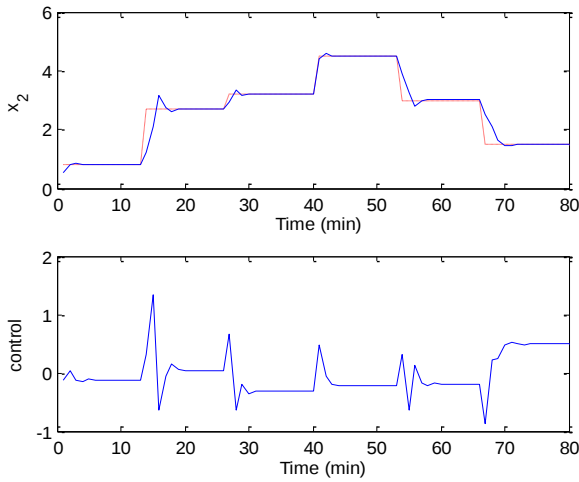
Fig. 5. Closed-loop response and control input moves of CSTR using two controllers.
