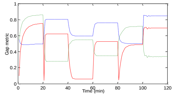
Fig. 9. Calculated gap metrics ((dotted) \delta_1 ; (solid) \delta_2 ; (dashed) \delta_3 )
