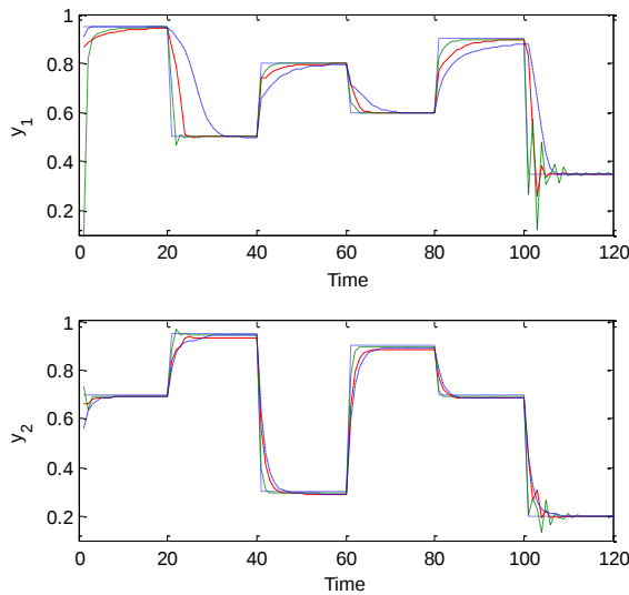
Fig. 10. Closed-loop response of TITO system using two controllers ((dotted) setpoint; (solid) with K_1 and K_2 ; (dashed) with K_2 and K_3 ; (dash-dotted) with K_1 and K_3 ).
