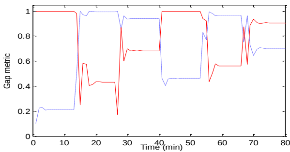
Fig. 6. Calculated gap metrics ((dotted) \delta_1 ; (solid) \delta_2 )
