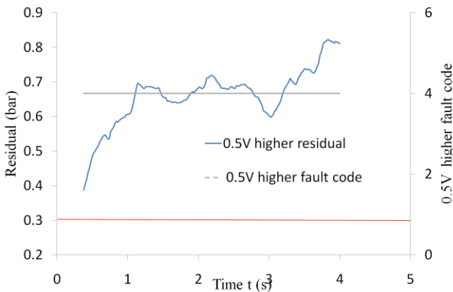
Fig. 10b. Curve of intake pressure of the sensor with 0.5V bias fault.
