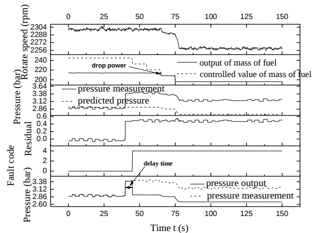
Fig. 16. Fault tolerance simulation of base fault
