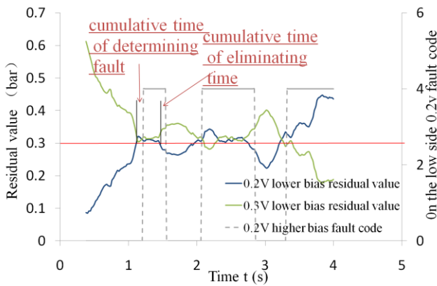
Fig. 10a. Curve of intake pressure of the sensor with 0.2V bias fault.
