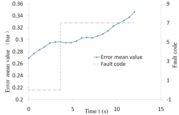
Fig. 11. Curve of intake pressure of the sensor with drift fault.
