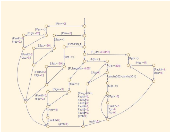
Fig. 14. Fault-tolerant control logic diagram
