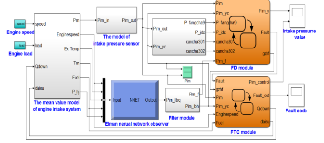
Fig. 13. FD_FTC system of diesel engine based on neural network observer.
