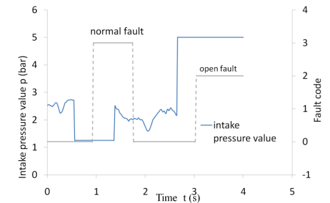
Fig. 9b. Curve of intake pressure of the sensor with open fault.
