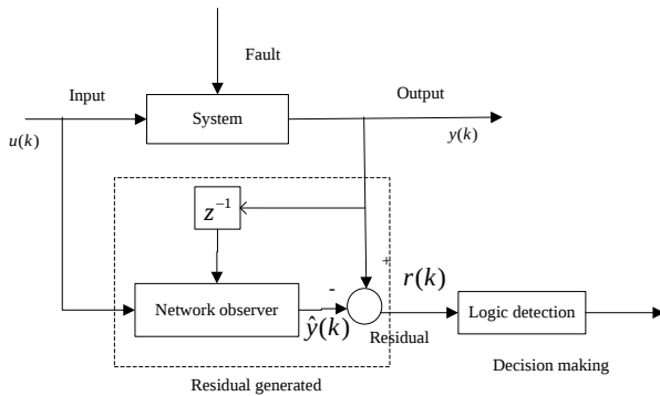
Fig. 3. Fault detection and isolation scheme based on neural network observer.
