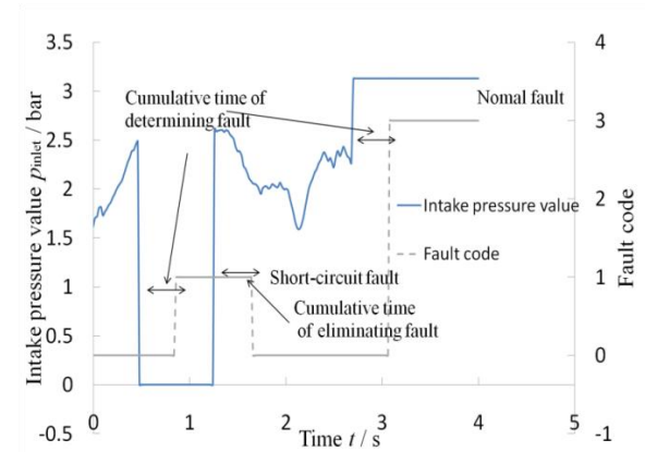
Fig. 9a. Curve of intake pressure of the sensor with normal fault.
