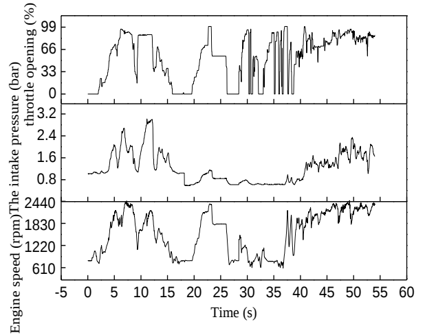
Fig. 4. Data of training samples.
