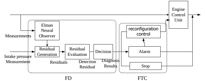
Fig. 1. Overview of the proposed FD–FTC system.
