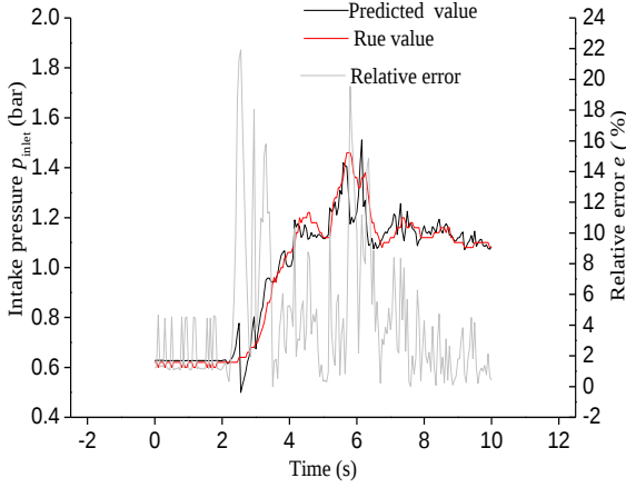
Fig. 8. Predicted results of sample 4.
