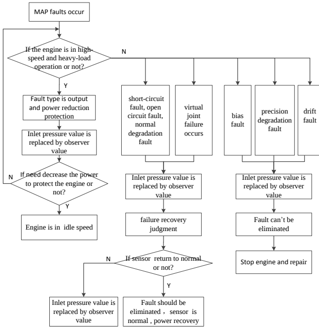
Fig. 12. Overview of proposed fault-tolerant control strategy
