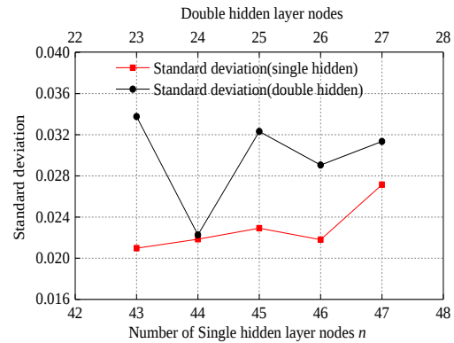
Fig. 7. Stability of the results using the Elman network with a single hidden layer nodes and double hidden layers, respectively.
