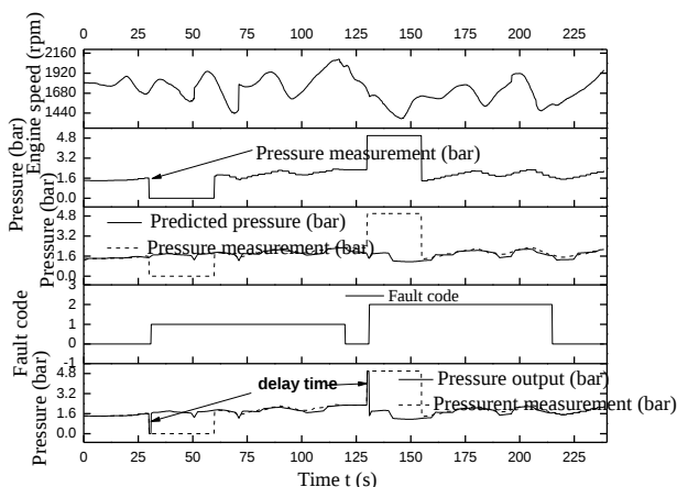
Fig. 15. Fault tolerance simulation of short circuit fault and open circuit
