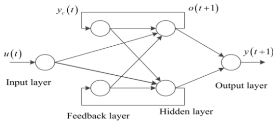
Fig. 2. Structure of an Elman neural network.
