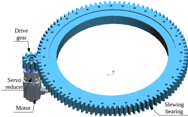
Fig.1 Simplified model of slewing bearing mechanical structure
