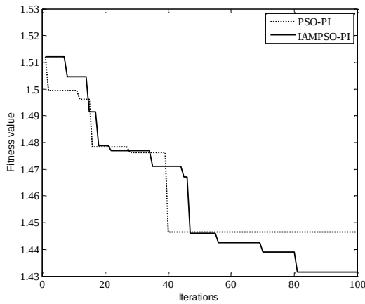
Fig.5 Fitness value evolutionary process
