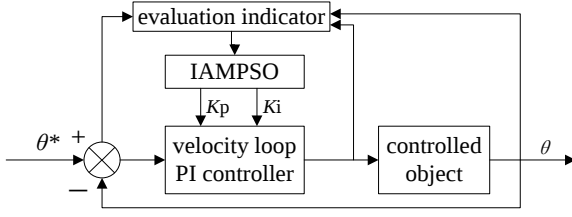
Fig.3 IAMPSO-PI controller
