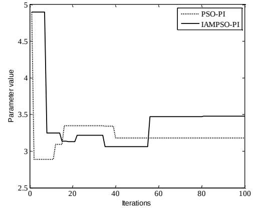
(a) K_p optimization process
