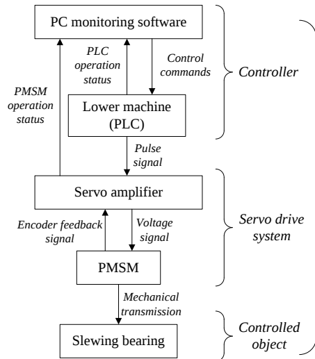
Fig.7 Slewing bearing motion control system
