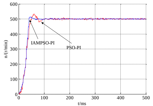
Fig.8 PMSM operation speed curve
