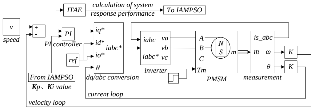
Fig.4 Simulation model of the system
