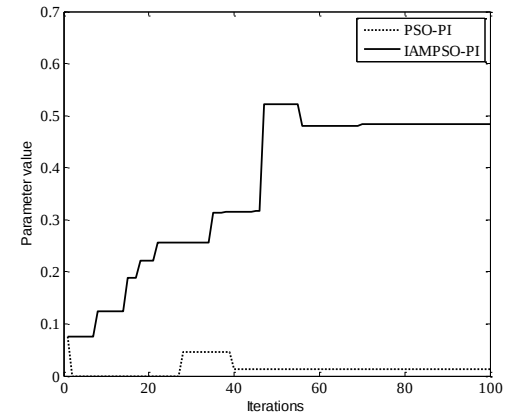
(b) K_i optimization process
