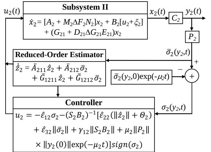
Fig. 3. Block diagram of the subsystem II
