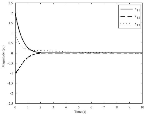
Fig. 4. Time responses of state x_{11} (solid), x_{12} (dashed), and x_{13} (dotted) of subsystem I
