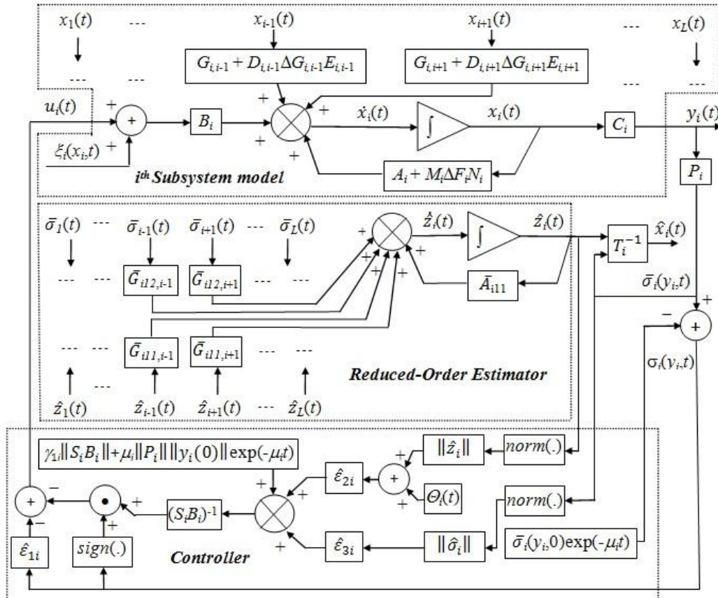
Fig. 1. Block diagram of the i^{\text{th}} subsystem
