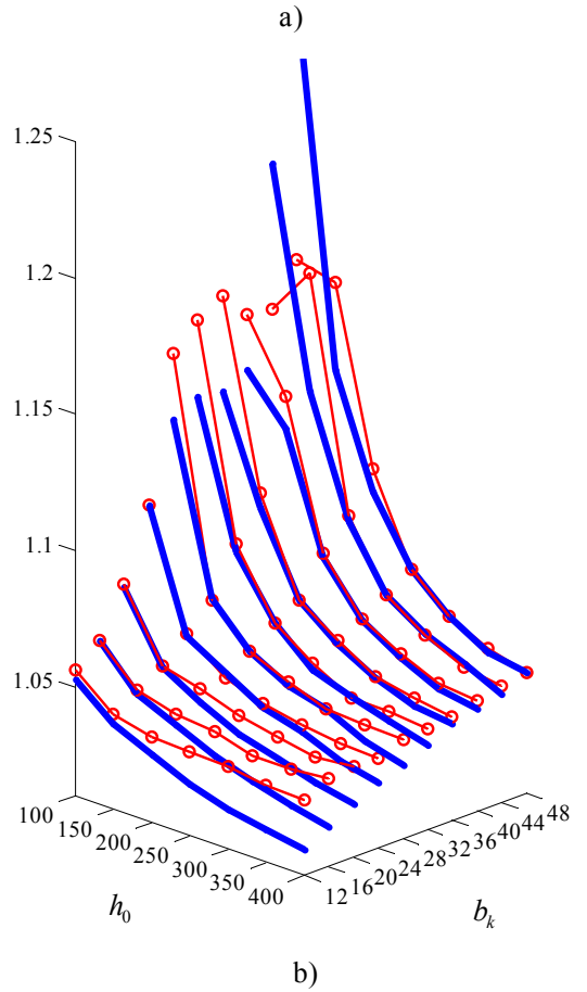
Fig. 3. Effects of applying the algorithm with values (20) best to be close to 1: bold lines stand for the optimal strategies, circled dots stand for 0.5's
