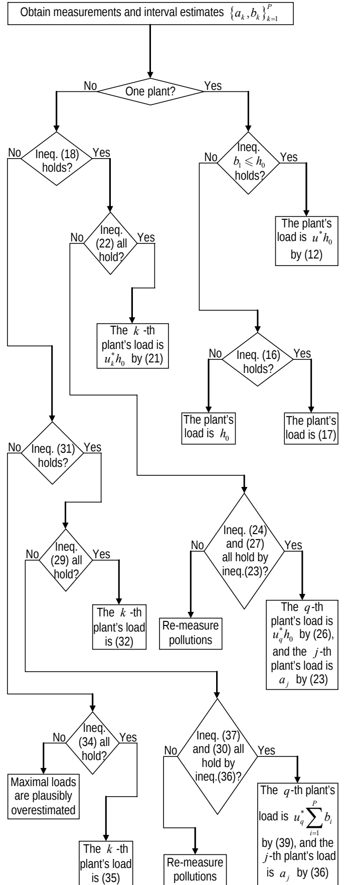
Fig. 1. Algorithm of distributing treatment loads
