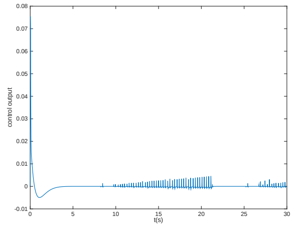
Fig.3. Control output
