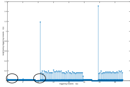
Fig.4. Event-triggering instants
