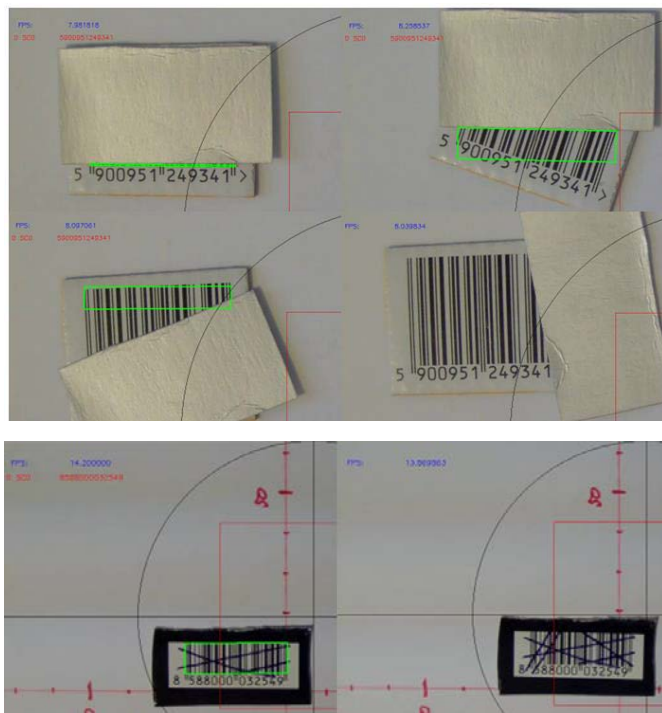
Fig. 14: Simulation of various corruptions of one-dimensional code
