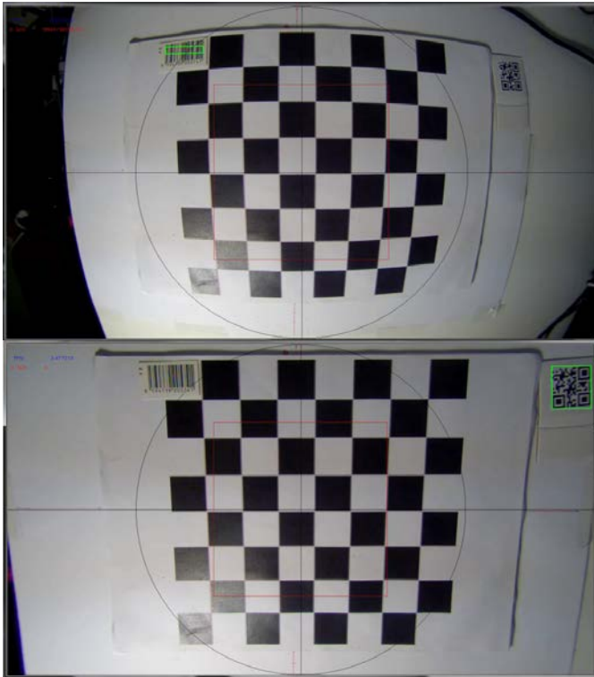
Fig. 7: Change of the detection capability after the distortion removal (left - without distortion, right - with eliminated distortion)
