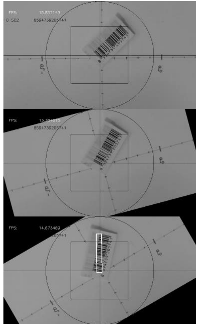
Fig. 3: Increase of probability of barcode detection by introducing rotated image detection
