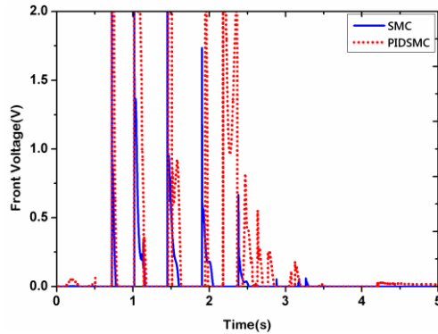
Fig.10. Input control voltage for MR-damper
