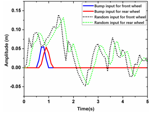
Fig.6. Road profiles
