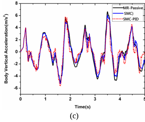
Fig.11. The time response of the system under excitation of random road. (a) SD, (b) FSWS and (c) BVA
