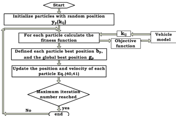
Fig.5. Steps in PSO algorithm
