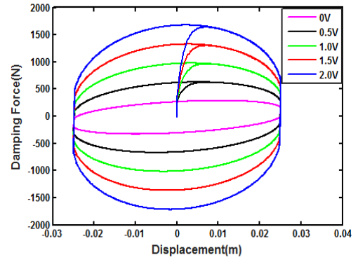
Fig.3. Characteristics of the MR damper
