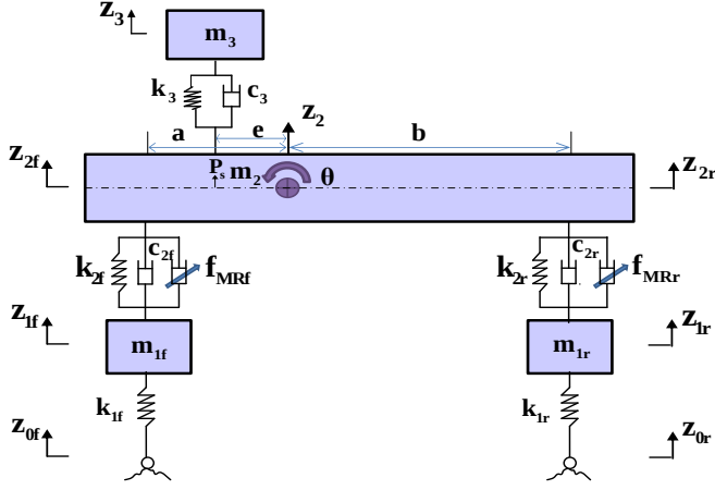
Fig.1. Half-car model with 5DOF
