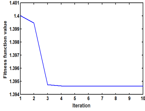
Fig. 8. The convergence characteristic of PSO-SMC-PID
