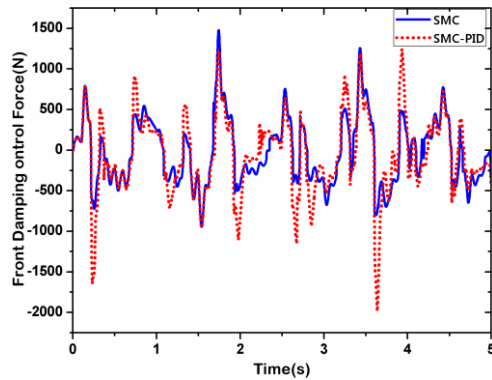
Fig.13. The control force of front wheel for RI
