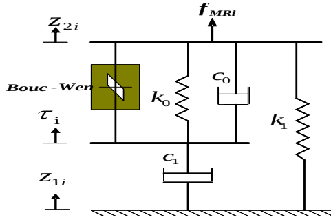
Fig.2. MR-damper model
