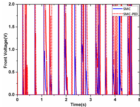
Fig.14. Input control voltage for MR-damper
