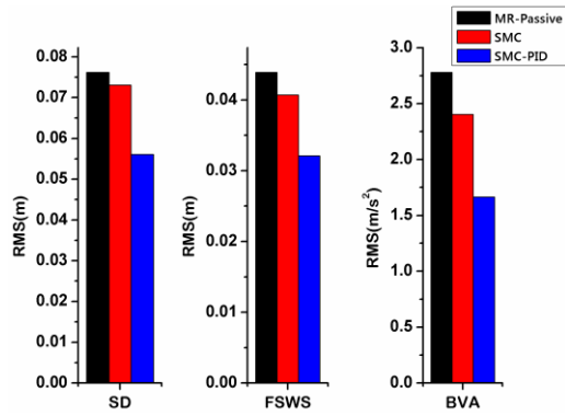
Fig.12. The RMS values of SD, FSWS and BVA of the system under RI road.
