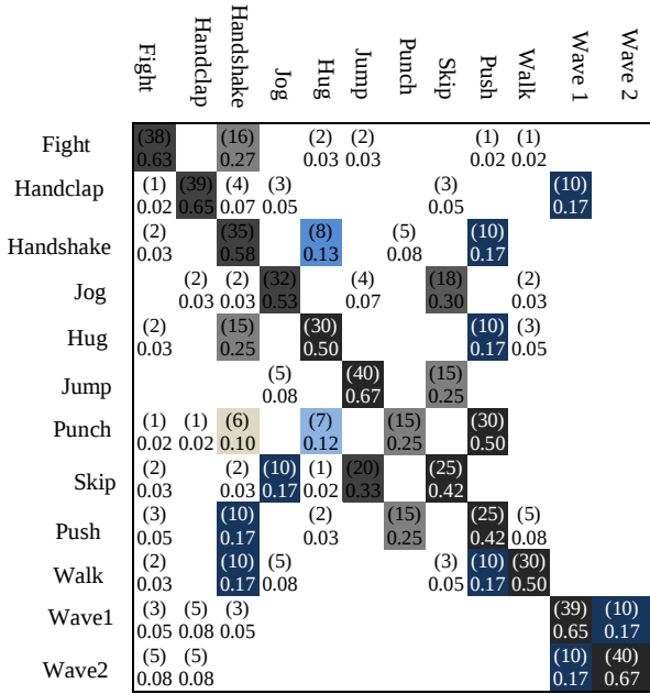
(a) Confusion matrix for unfiltered test and training data
