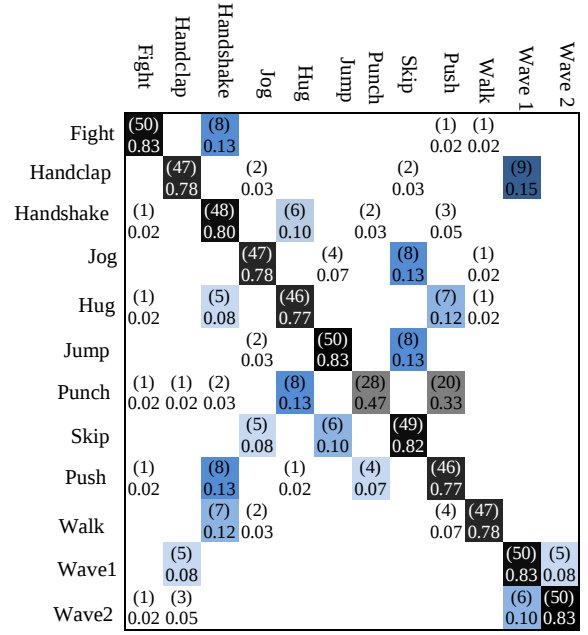
(b) Confusion matrix for the training data filtered
