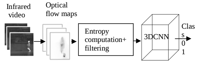
Fig. 1.General structure of the proposed approach
