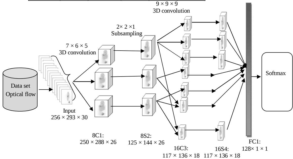
Fig 3. 3D CNN global architecture applied for human action recognition
