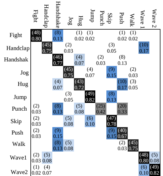
(c) Confusion matrix for filtered test data
