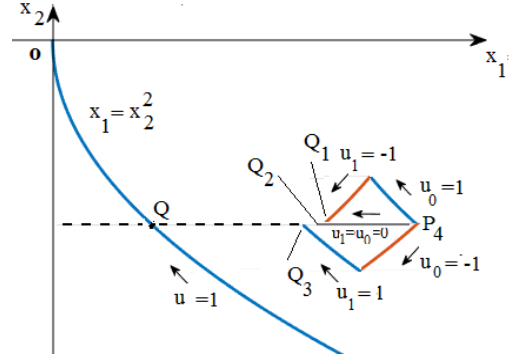
Fig. 4. Alternative state trajectories for the system (13) evolution being initially in state P_3 .
