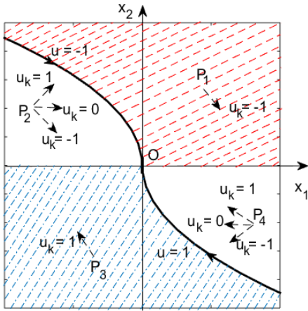
Fig. 3. Curved regions, generic points and evolution tendencies of states for every region.
