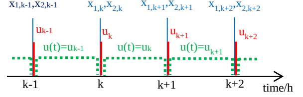
Fig. 14. Control signal generation for an ideal digital system.
