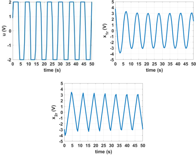
Fig. 18. The behavior of the system in Fig.17 in case \alpha = 0 (time delay is not compensated). Signals u , x_{1r} and x_{2r} are taken from points (7), (1), respectively (2).
