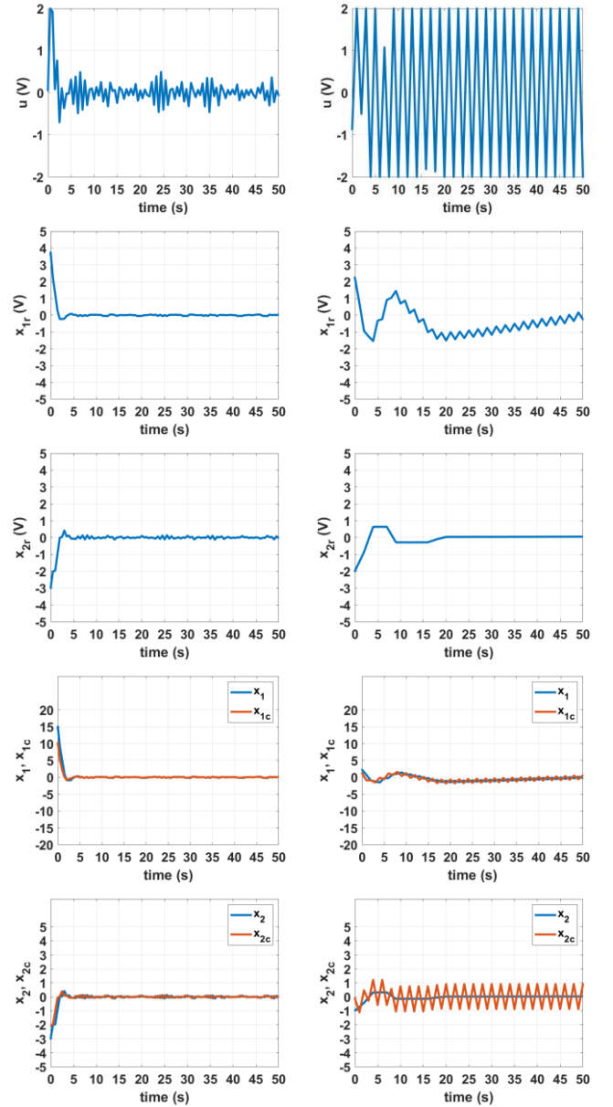
Fig. 20. The behavior of the system in Fig. 17 in case \alpha = 0.95 , h=0.5 (left diagrams) and \alpha = 0.9 , h = 1 s (right diagrams). The signals u , x_{1r} , x_{2r} , x_{1c} , x_{2c} are obtained from the points (7), (1), (2), (3), (4), (5), (6).
