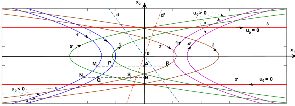
Fig. 1. Simple state trajectories of system (2) when u(t)=u_0 \cdot \{1, 1', 2, 2'\} for u_0 < 0 , \{3, 3'\} for u_0 = 0 , and \{4, 4', 5, 5'\} for u_0 > 0 .
