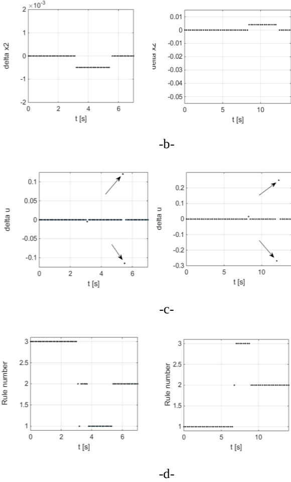
Fig. 12. Comparisons in Case 1 (left) and Case 2 (right) between the D-RBOC (25) and D-RBOC (28) with a=0.5 .
