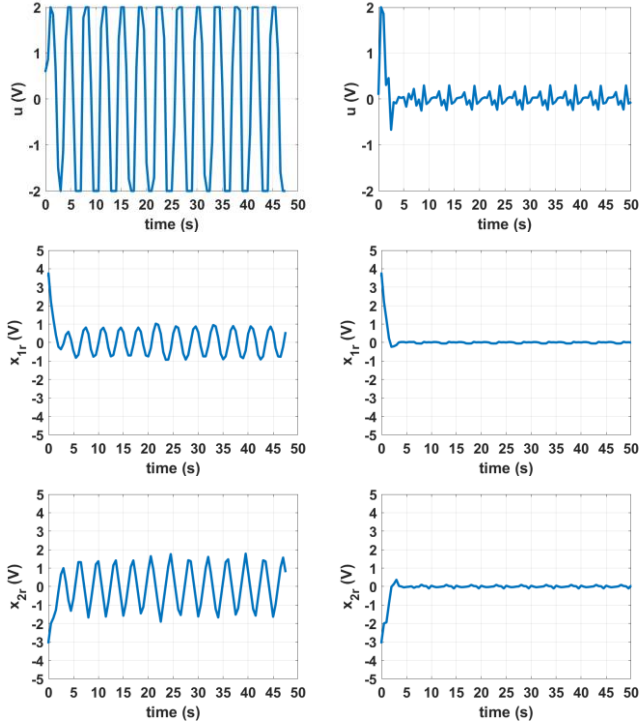
Fig. 19. The behavior of the system in Fig.17 in cases \alpha = 0.4 (left) and \alpha = 0.9 (right). The signals u , x_{1r} and x_{2r} are obtained from the points (7), (1), respectively (2).
