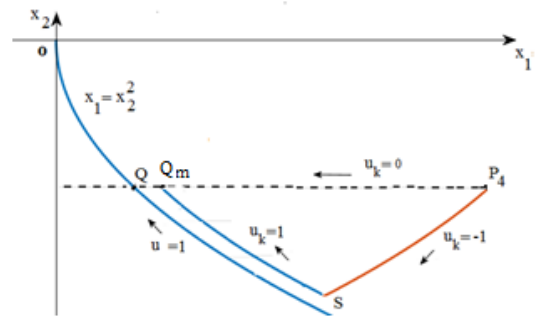
Fig. 5. State trajectory P_4SQ_m when control (18) is applied.
