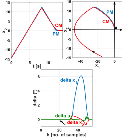
Fig. 11. The comparison of the effect of PM and CM algorithms in case 2 from Fig. 8
