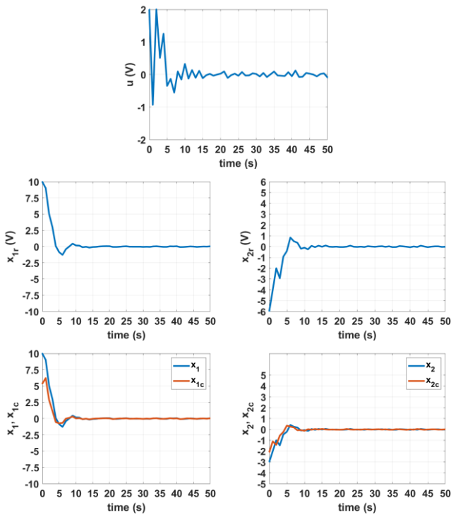
Fig. 21. The behavior of the system in Fig. 17 in case \alpha = 0.475 , h = 1 s. Signals u , x_{1r} , x_{2r} , x_1 , x_2 , x_{1c} and x_{2c} are taken in points (7), (1), (2), (3), (4), (5), respectively (6).
