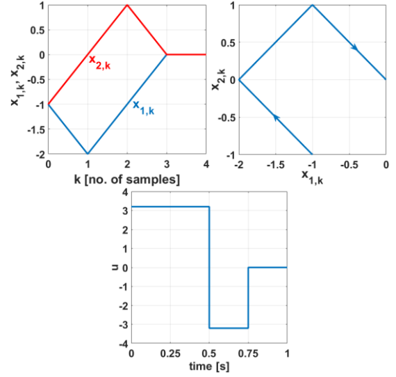
Fig. 9. In case 3 the control laws PM and CM lead to identical results.
