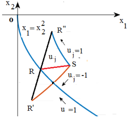
Fig. 6. Possible evolutions from point S when control u_j \in [-1, 1] is applied.
