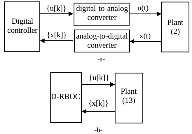
Fig. 7. The structure of the minimal time control system
