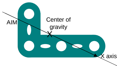
Fig. 3 Object-attached frame for general use
