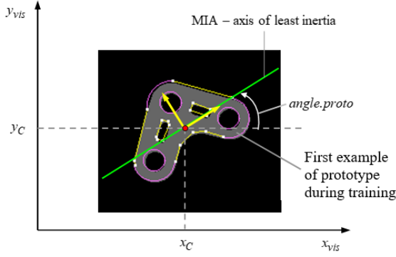
Fig. 4. – Best fit line segments and arcs for a gear's boundary. Region 1 (body) is approximated by 7 lines and 3 arcs. Regions 2-6 (holes) are defined by a total of 10 lines and 3 arcs. The object's frame ( x_c, y_c, angle.proto ) is shown, C - mass centre.
