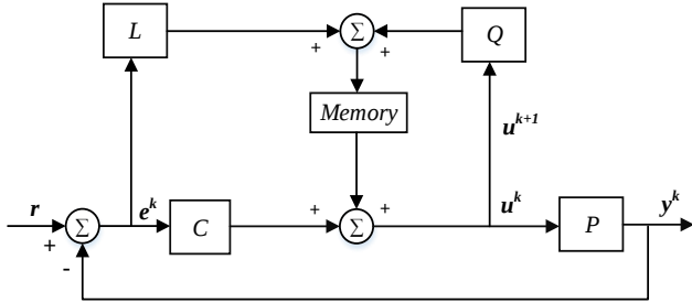
Fig.3. ILC Configuration structure with feedback
