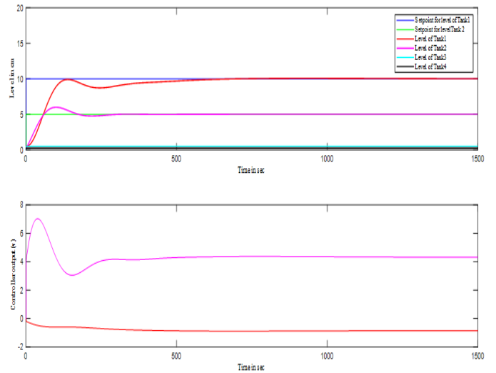
Fig.6. Responses of PI controller without Decoupler under non-minimum phase condition
