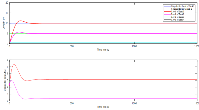
Fig.7. Responses of PI controller with Decoupler under minimum phase condition
