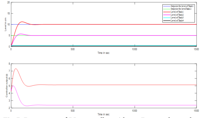
Fig.5. Response of PI controller without Decoupler under minimum phase condition
