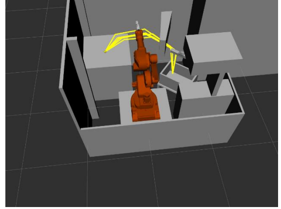
Fig. 15. Failure of STOMP, which used parameters from previous experiment. Noise is too low, and solver cannot find trajectory.
