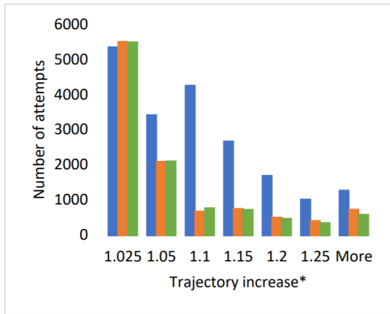
Fig. 14. Comparison STOMP (blue), RRTConnect (orange), RRT (green) by histogram, which shows number of attempts on intervals with different trajectory increase.
