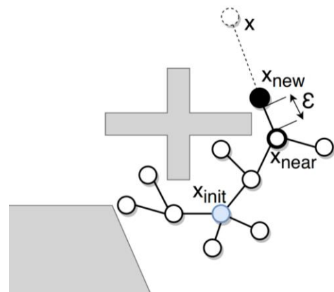
Fig. 2. Example of one iteration of RRT.
