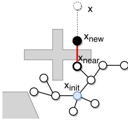
Fig. 3. Example of connection failure.
