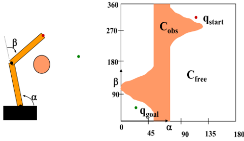
Fig. 1. Configuration space, \mathcal{C}_{free} and \mathcal{C}_{obs} for an articulated robot with two joints (Gasparetto et al., 2015)
