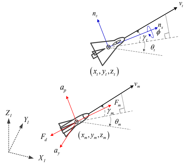
Fig. 1. Mathematical models of target and missile dynamics.
