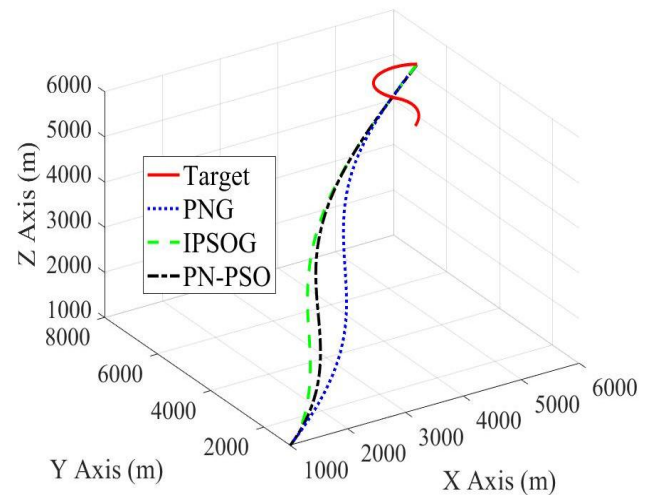
Fig. 12. Interception trajectories of missile using PN-PSO, IPSOG, and PNG against a highly maneuverable evasive target in Scenario III.
