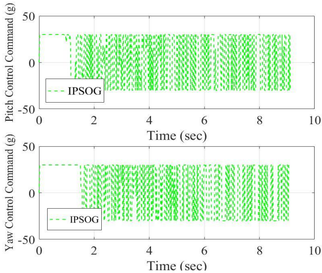
Fig. 10. Variation of missile control commands over time for IPSOG in Scenario II.
