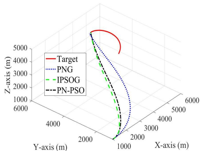
Fig. 8. Interception trajectories of missile using PN-PSO, IPSOG, and PNG against a big G-force turning target in Scenario II.
