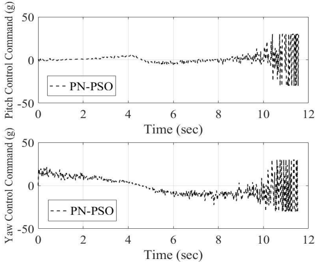
Fig. 13. Variation of missile control commands over time for PN-PSO in Scenario III.
