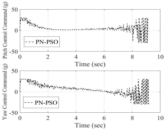
Fig. 9. Variation of missile control commands over time for PN-PSO in Scenario II.
