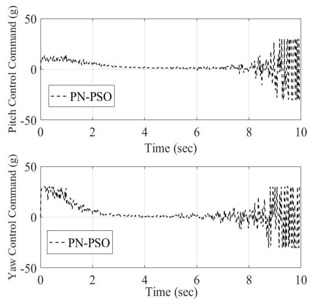
Fig. 5. Variation of missile control commands over time for PN-PSO in Scenario I.
