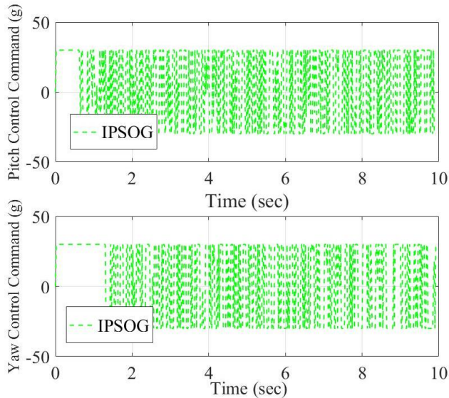
Fig. 6. Variation of missile control commands over time for IPSOG in Scenario I.
