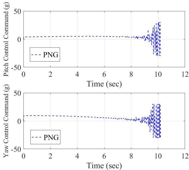
Fig. 7. Variation of missile control commands over time for PNG in Scenario I.
