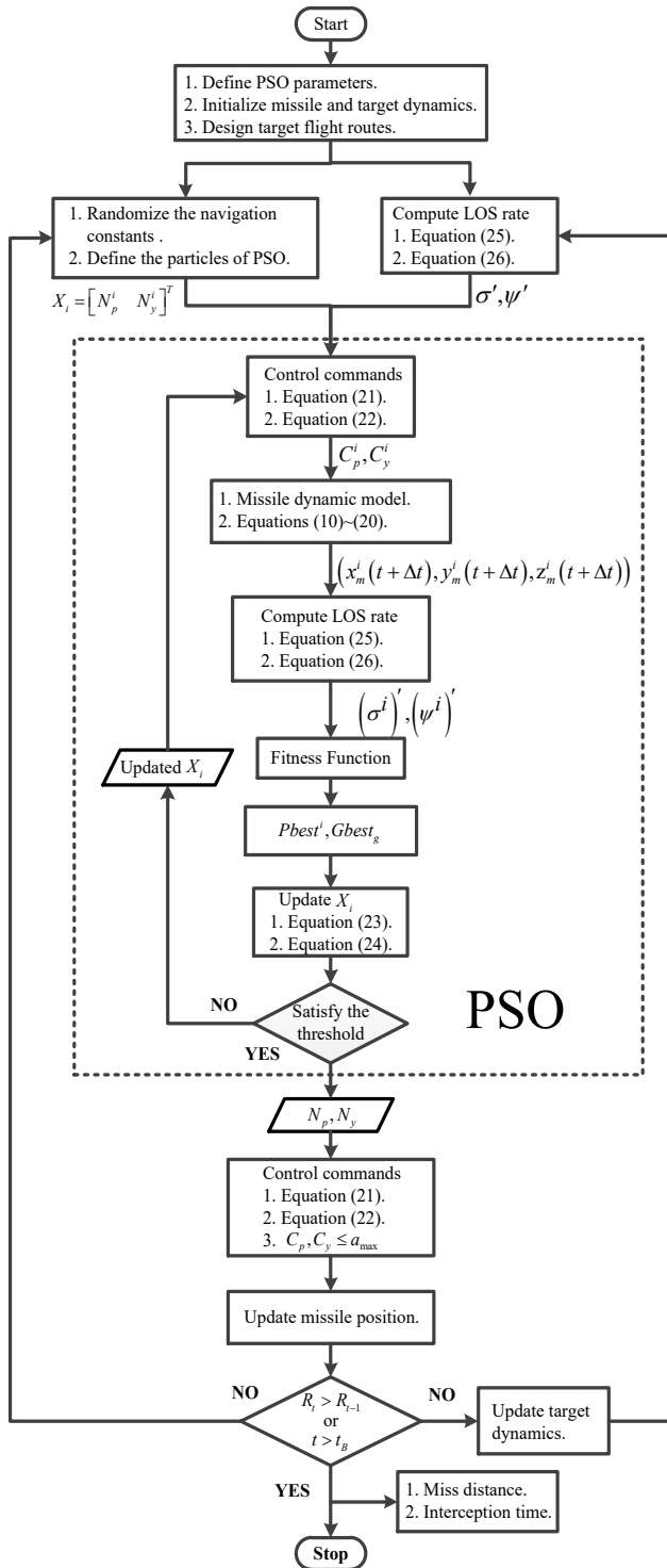
Fig. 3. Flow chart of the proposed PN algorithm.
