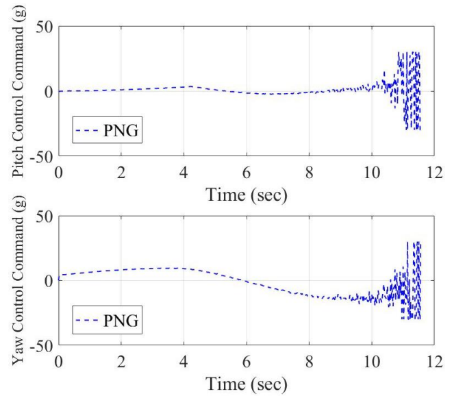
Fig. 15. Variation of missile control commands over time for PNG in Scenario III.
