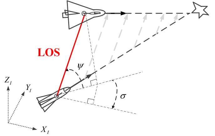
Fig. 2. Illustration of PN mode.
