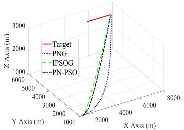
Fig. 4. Interception trajectories of missile using PN-PSO, IPSOG, and PNG against a nearly straight-line target in Scenario I.
